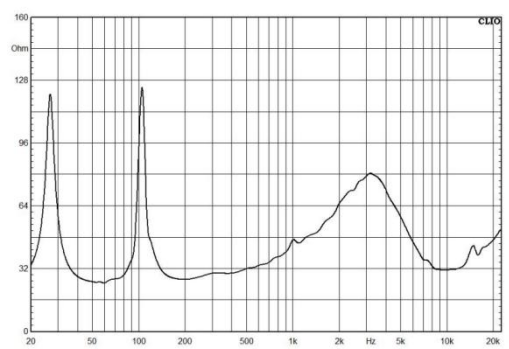
Impedance Curve (Constant Voltage)
