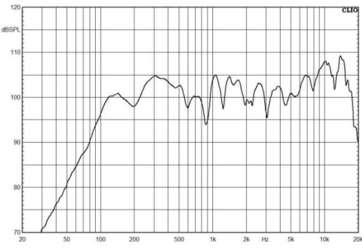
Frequency Response (dB SPL, 1W, 1m)
